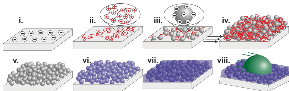
Figure 1. Schematic illustration of the layer-by-layer process to form nanoscale slippery, lubricant-infused porous coatings (LbL SLIPS). Negative charges are introduced to the substrate (i) and subsequent layers of positively charged polyelectrolyte (ii) and negative charged silica nanoparticles (iii) are adsorbed to form a hybrid thin film (iv) that can be calcined to produce a porous silica coating (v). After covalently functionalizing the surface with fluorinated silanes (vi), a fluorinated lubricant is wicked into the coating (vii), rendering the surface non-adhesive and allowing for a secondary immiscible liquid to slide off the substrate with ease (viii).
