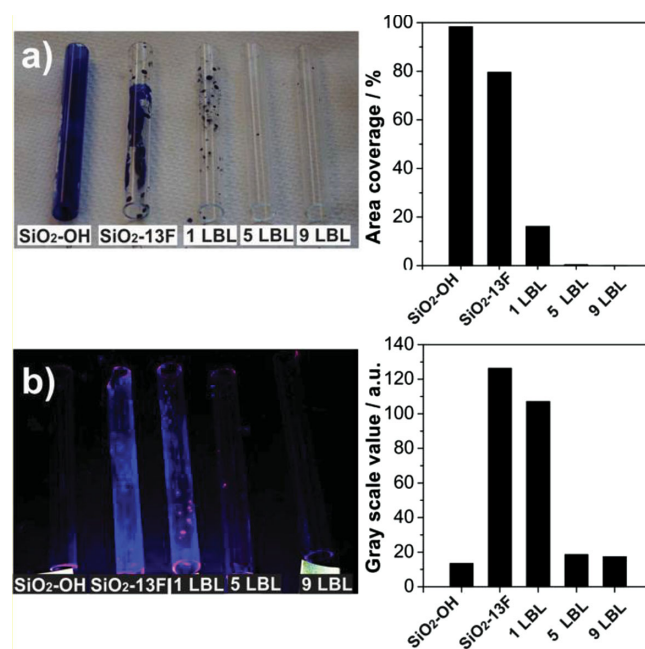
Figure 8. Adhesion and staining of LbL coated, lubricant-infused tubes. Tubes coated with different numbers of nanoparticle layers were subjected to water flow (10 mL/min) for 24 h and then stained with a water-soluble, commercial blue dye (Dharma Pigment 60 Blue Dye) (a) and fluorescently labelled streptavidin proteins (b). Tubes coated with 5 and 9 nanoparticle layers showed negligible staining and a significant decrease in protein adsorption.
