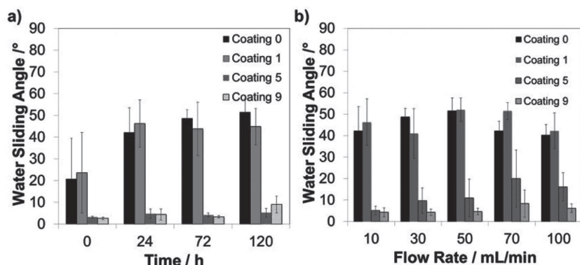
Figure 7. Performance of lubricant-infused LbL coatings under flow. Glass tubes coated with different numbers of nanoparticle layers and infused with a fluorinated lubricant (Krytox 103) were subjected to a continuous flow of water with a flow rate of 10 mL/min for different times (a) and with different flow rates for 24 h (b). After the flow was stopped, the water was drained and the sliding angles of individual droplets of water (70 \mu L) recorded to investigate if the coating retained its repellency properties. Coatings with 9 deposited silica nanoparticle layers retained water repellency for all tested times and flow rates.
